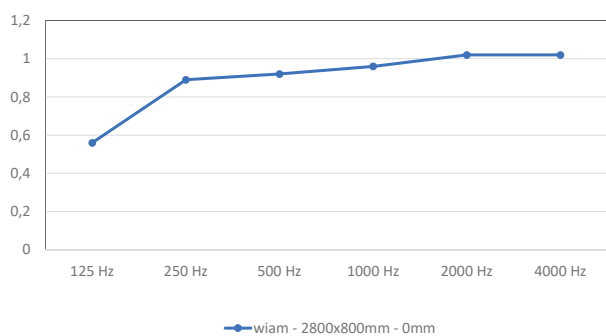
Schallabsorptionsgrad alpha s
